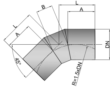
45° ELBOW, 2-MITER
